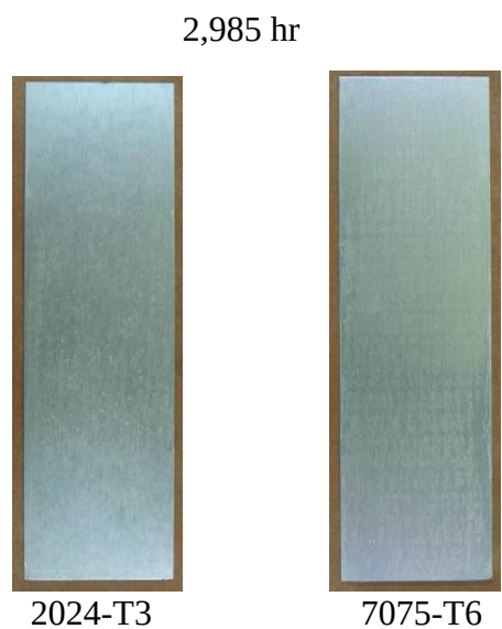
Figure 17: TCP Sealed Metalast Type IIB Anodize Coatings Exposed to NSF for 2,985 hr
